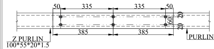
PURLINS OVER LAP DETAIL
