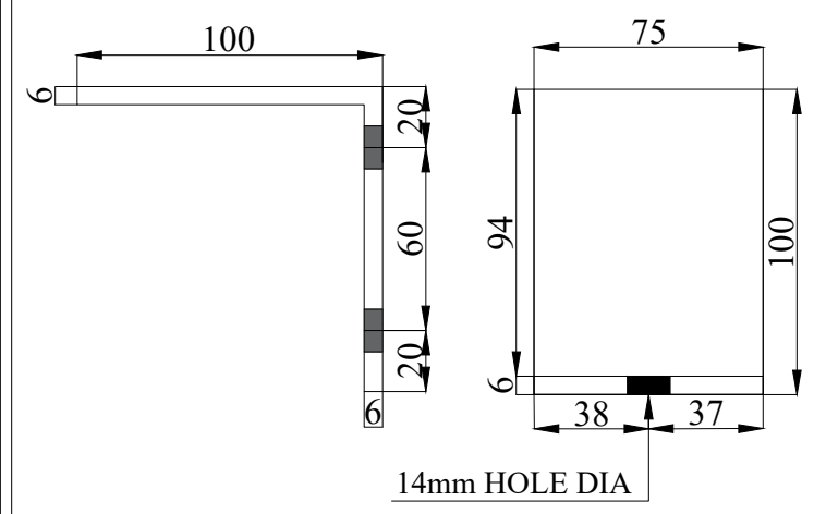
DETAIL OF [L-CLIP-100*100*75*6]
