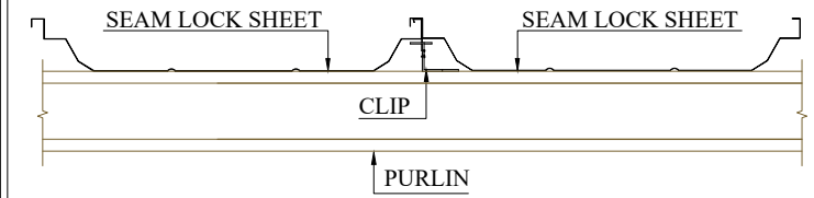
PURLIN WITH SEAM LOCK CLIP DETAIL
