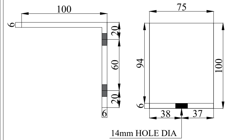
DETAIL OF [L-CLIP-100*100*75*6]
