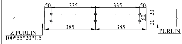
PURLINS OVER LAP DETAIL
