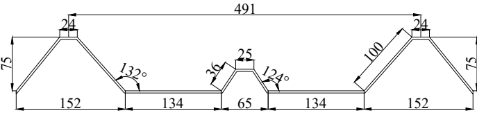
SKYLIGHT PROFILE : THK. 2mm
