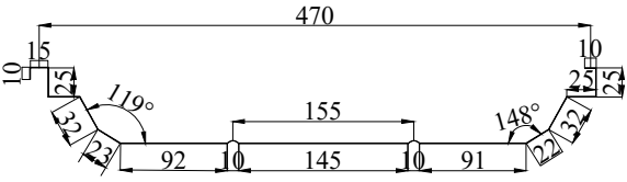
LOCK SEAM SHEET PROFILE
