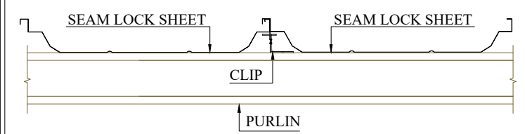
PURLIN WITH SEAM LOCK CLIP DETAIL
