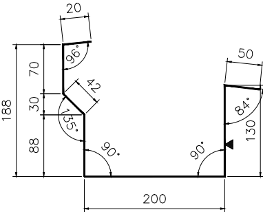
EAVE GUTTER
